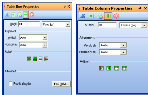
Row properties
